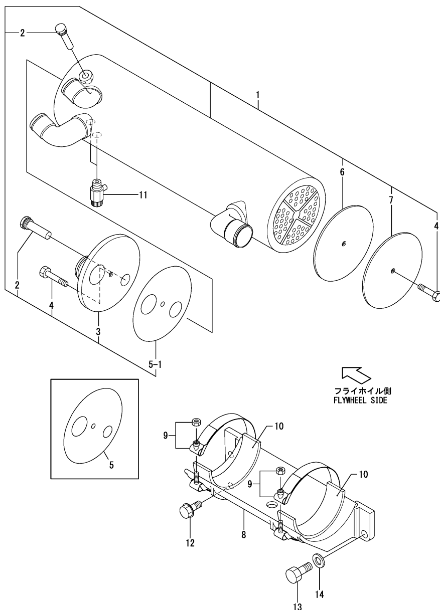
Fig.34. COOLER(FRESH WATER)
