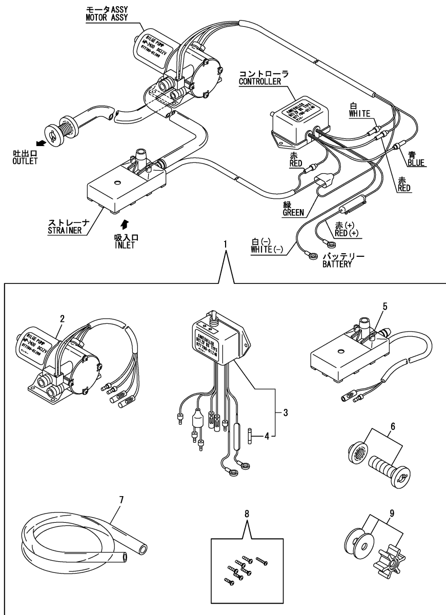
Fig.25. BILGE PUMP(DX)(OPTIONAL)
