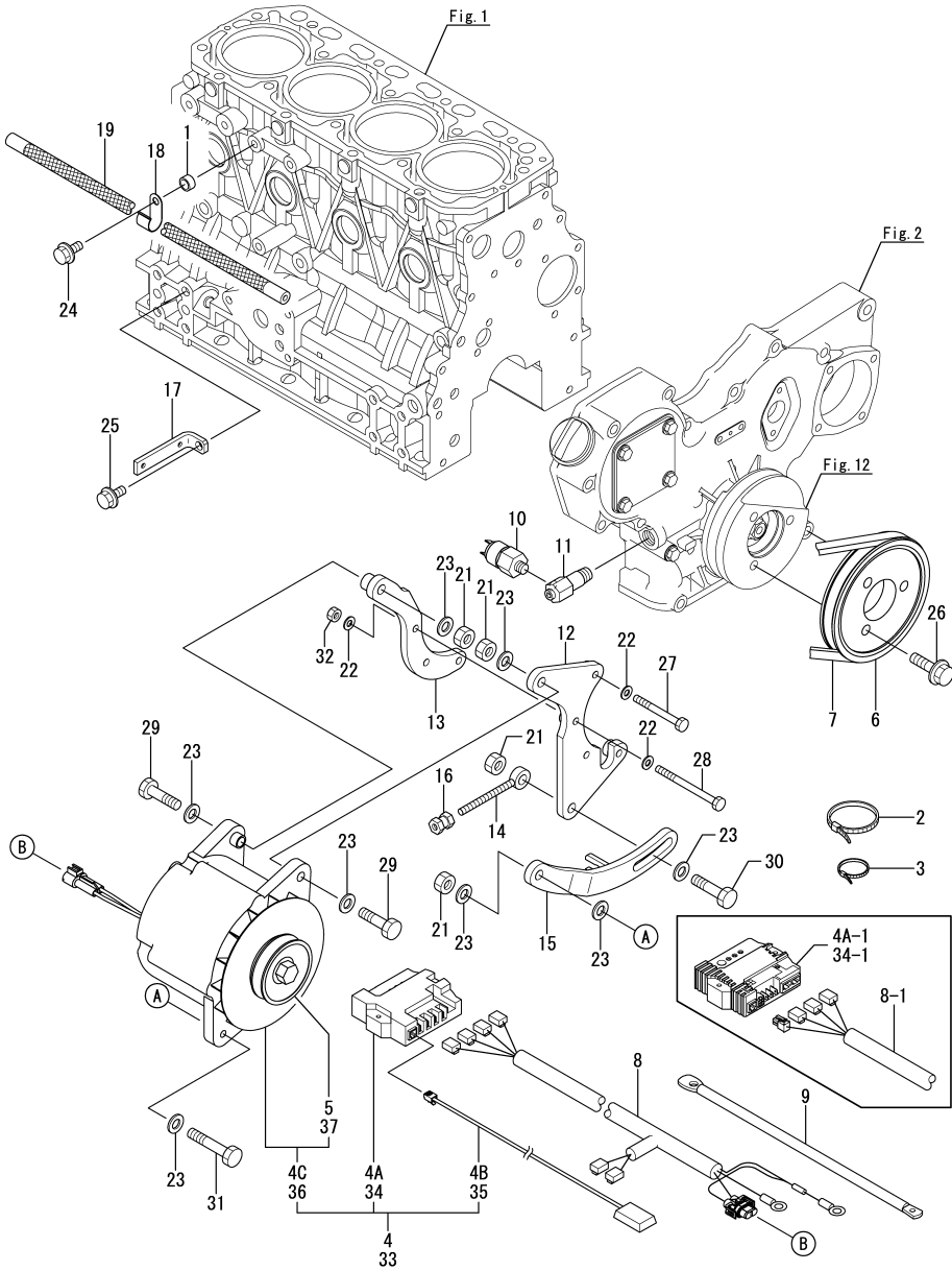
Fig.46. GENERATOR(ADDITION) & GENERATOR MOUNT PART(OPTIONAL)
