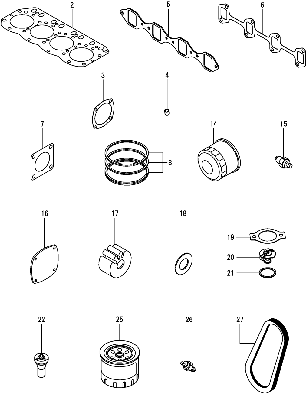
Fig.50. SPARE PARTS KIT(OPTIONAL)
