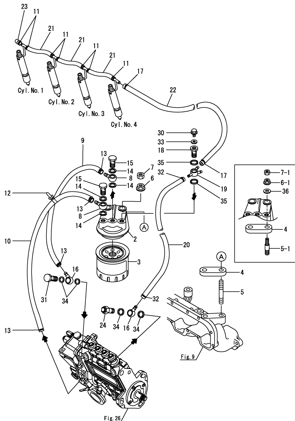
Fig.31. FUEL PIPE & FUEL STRAINER
