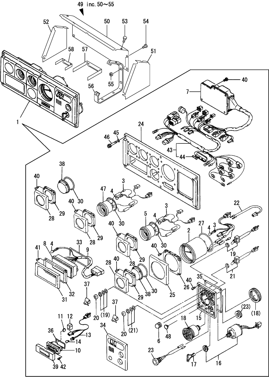
Fig.39. INSTRUMENT PANEL(4LH-WST)
