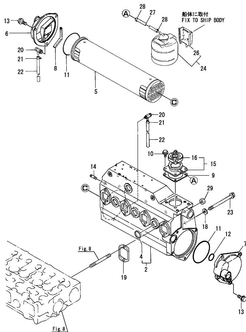
Fig.20. FRESH WATER COOLER & COVER
