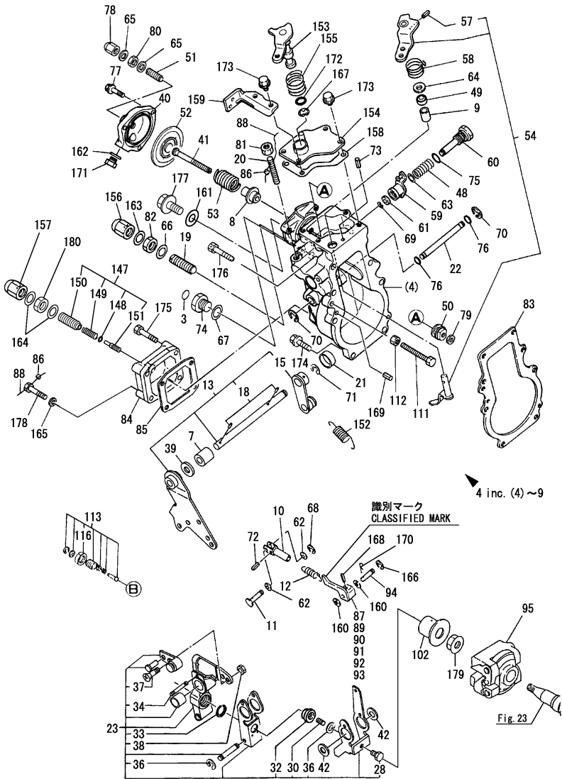
Fig.24. GOVERNOR
