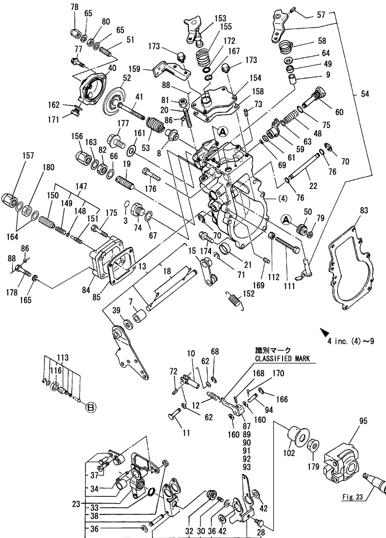
Fig.24. GOVERNOR
