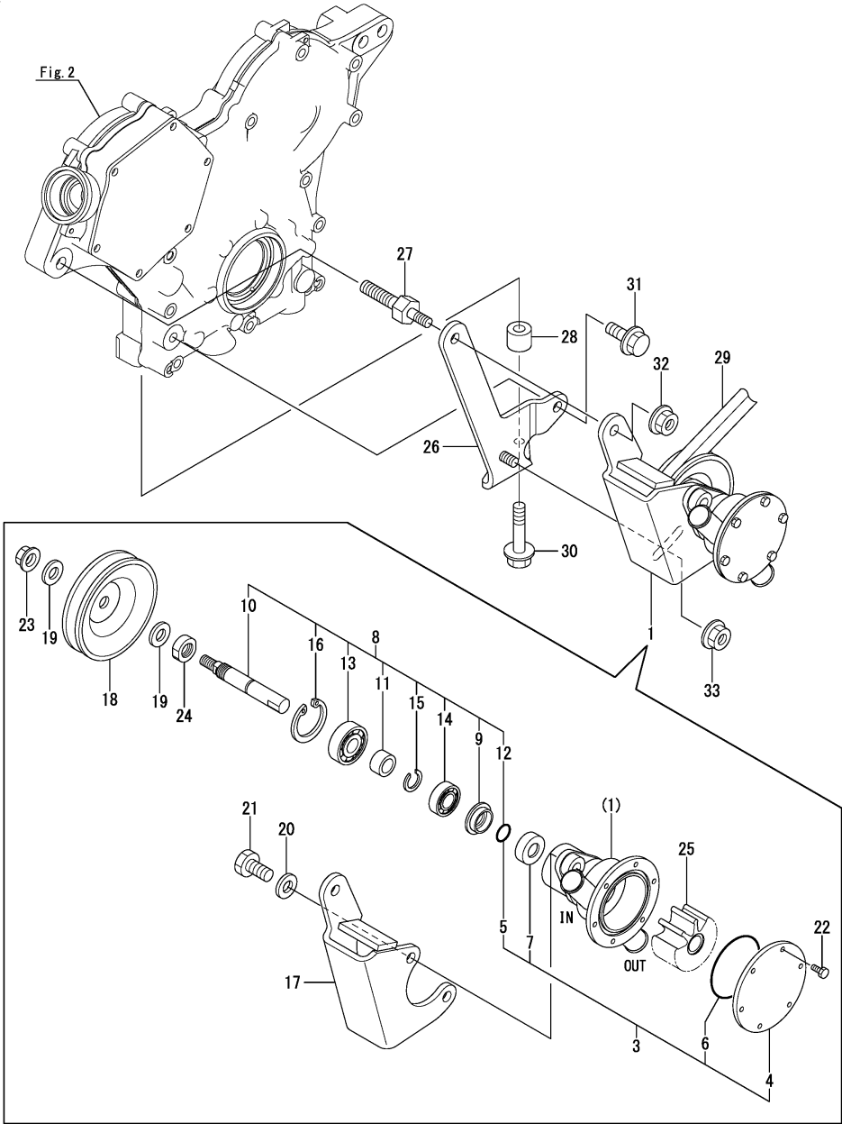
Fig.16. COOLING PUMP(SEA WATER)
